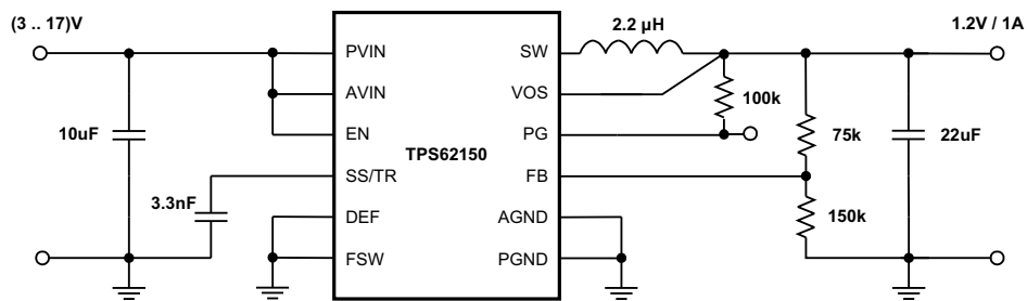
Figure 52. 1.2-V, 1-A Power Supply
