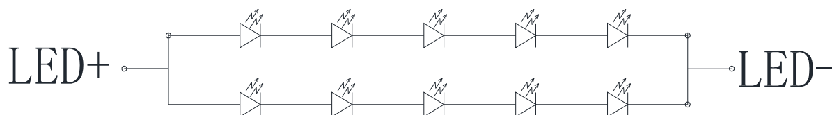
CIRCUIT DIAGRAM
