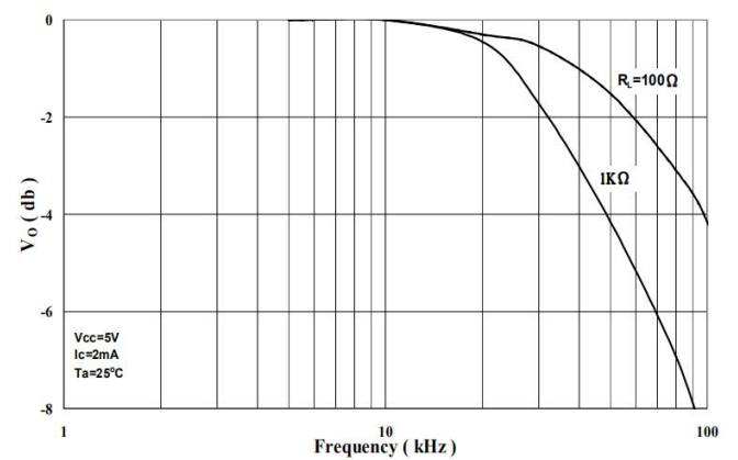
Figure 18. Frequency Response
