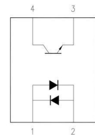
1. Anode, Cathode 3. Emitter 2. Cathode, Anode 4. Collector
