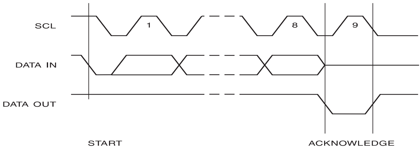
Figure 6. Output Acknowledge
