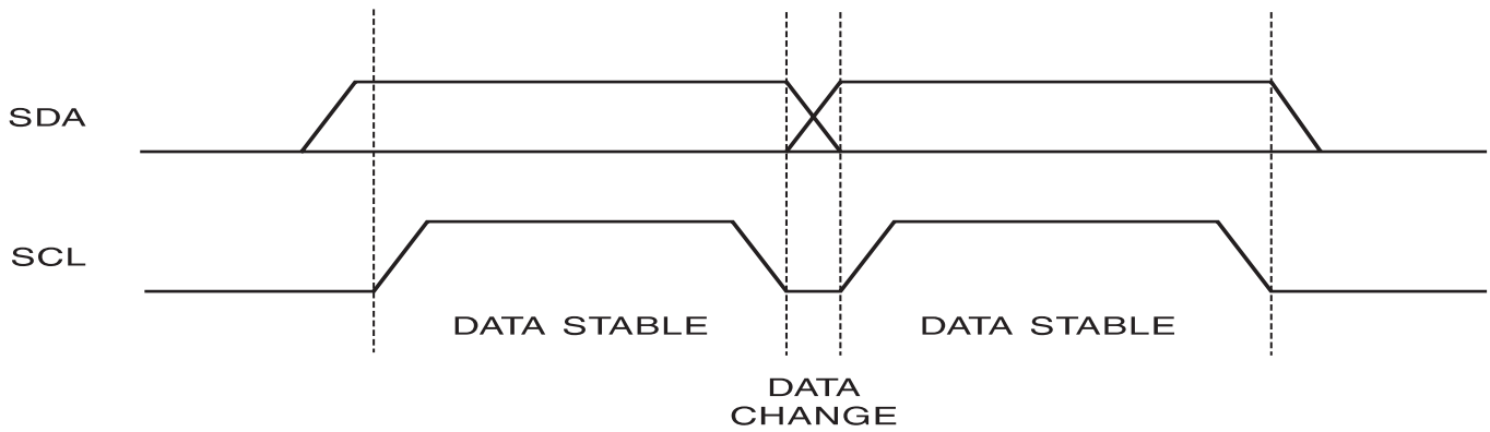
Figure 4. Data Validity
