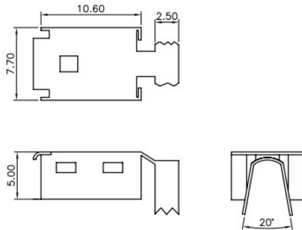
Upper shell
