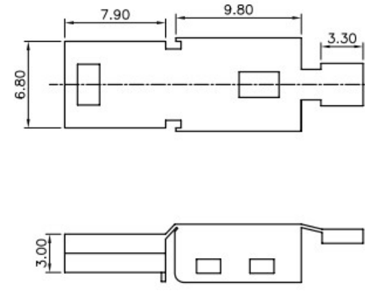
Down shell
