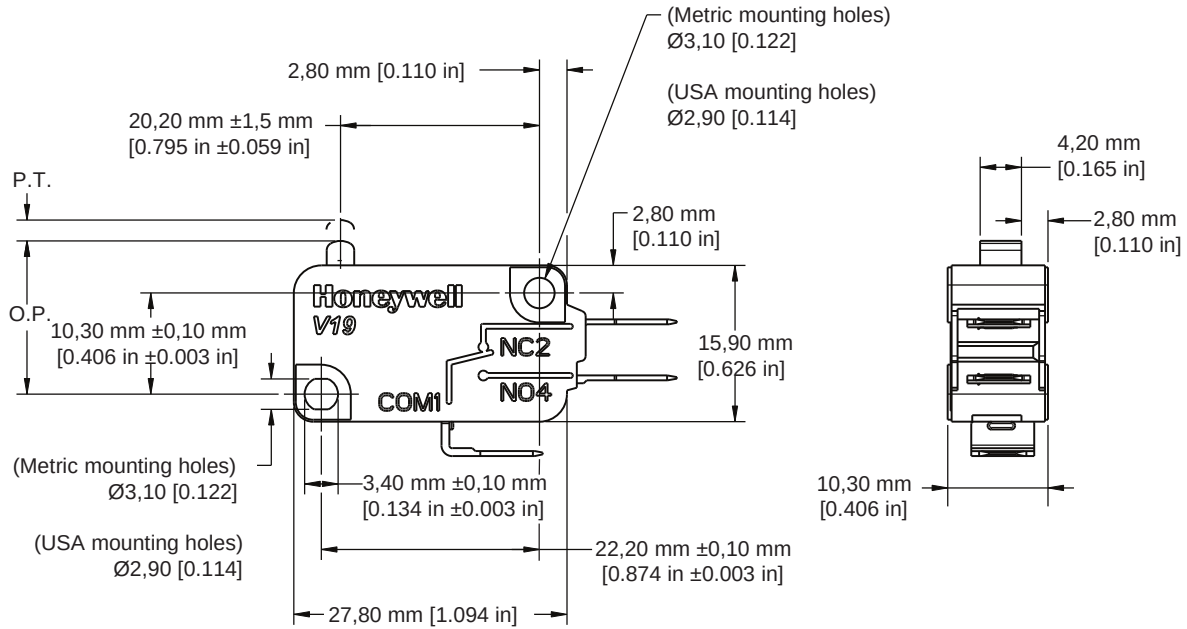
FIGURE 4. V19 SERIES HOUSING DIMENSIONS
