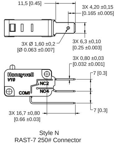
FIGURE 9. V19 SERIES N-STYLE RAST-7 250# CONNECTOR
