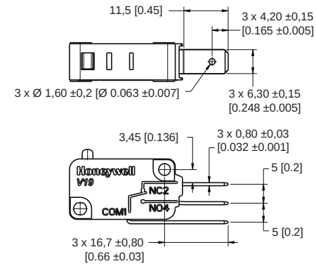
FIGURE 7. V19 SERIES H-STYLE RAST-5 250# CONNECTOR
