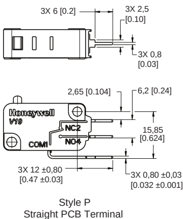
FIGURE 10. V19 SERIES P-STYLE STRAIGHT PCB TERMINAL
