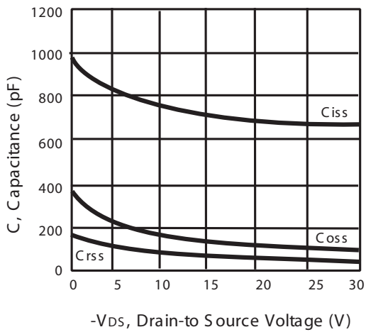
Figure 3. Capacitance
