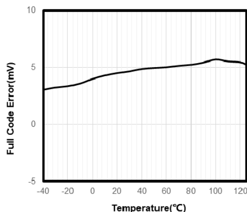
Full-Scale Error vs. Temperature (TPC112S1)
