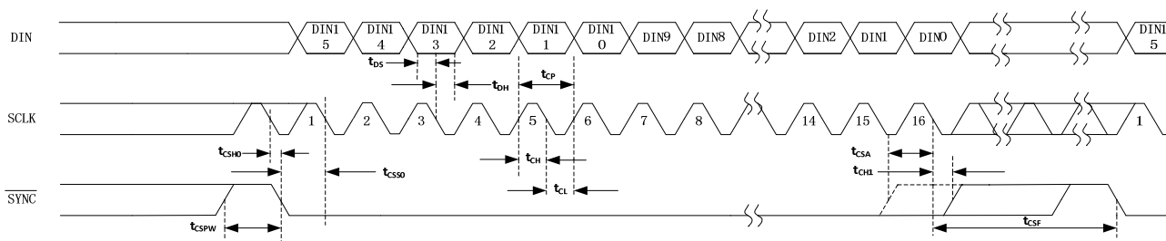
Figure 1. 16-Bit Serial-Interface Timing Diagram (TPC112S1)
