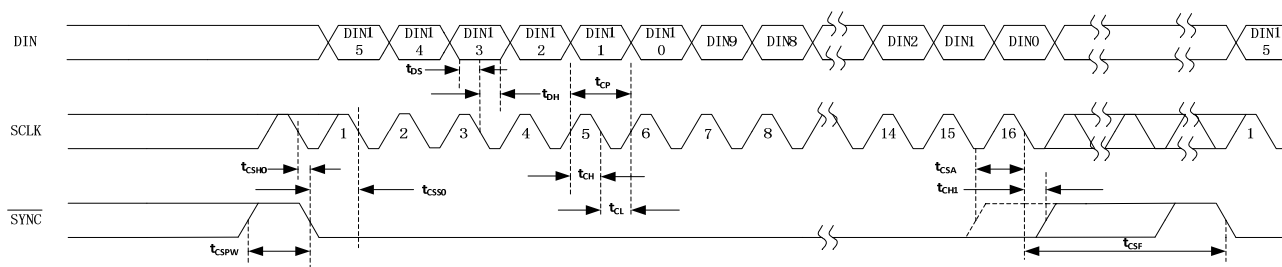
Figure 2. 16-Bit Serial-Interface Timing Diagram (TPC114S1)
