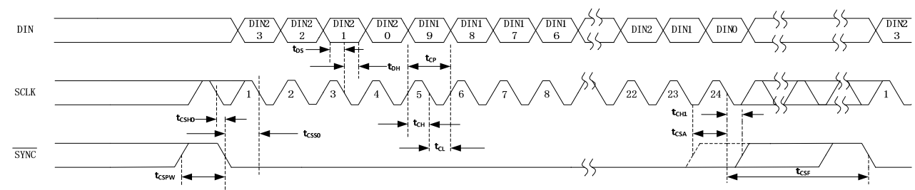
Figure 3. 24-Bit Serial-Interface Timing Diagram (TPC116S1)
