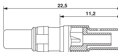
D-SUB coaxial contact socket
