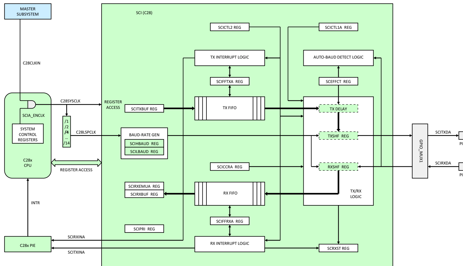
Figure 5-50. SCI (C28x)
