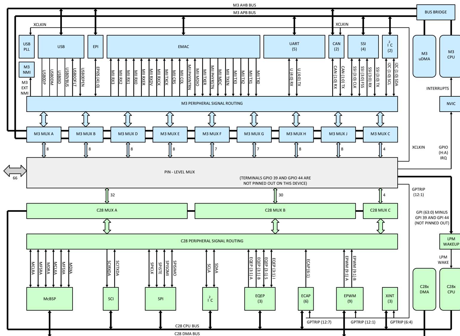
Figure 6-15. GPIO_MUX1 Block
