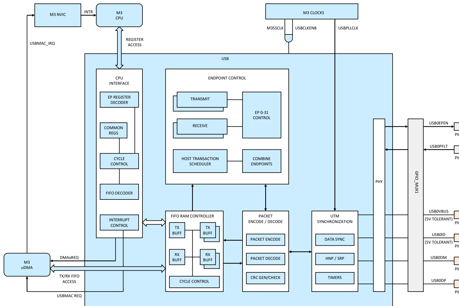
Figure 5-35. USB
