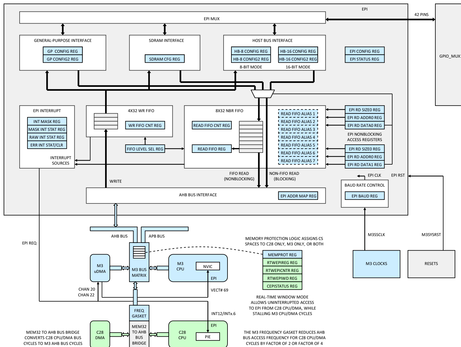
Figure 5-17. EPI
