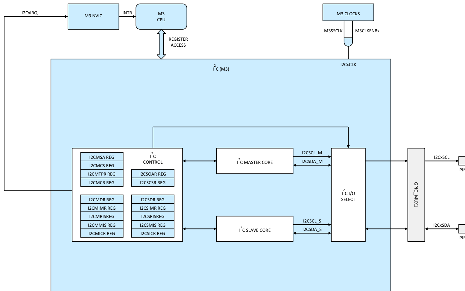
Figure 5-33. I2C (Cortex-M3)
