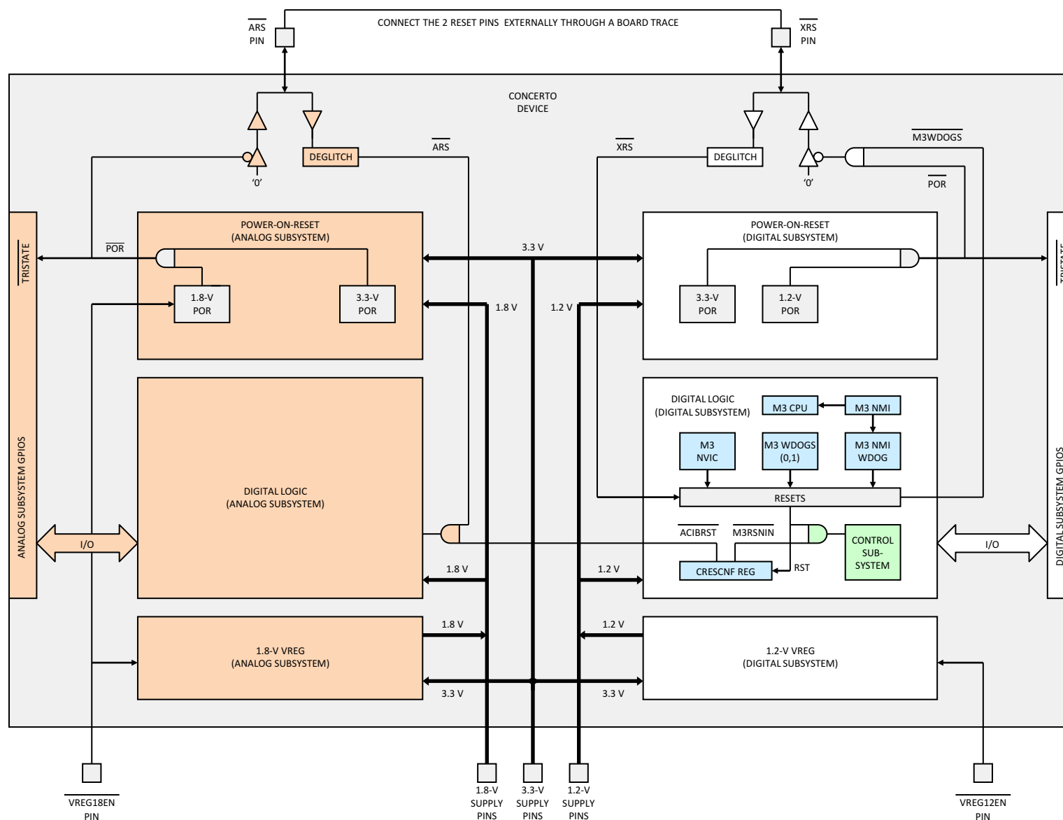
Figure 6-6. Voltage Regulation and Monitoring
