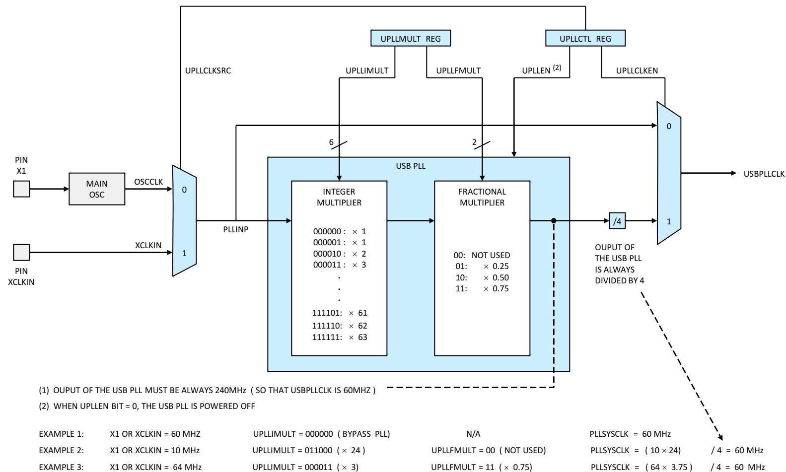
Figure 6-9. USB PLL
