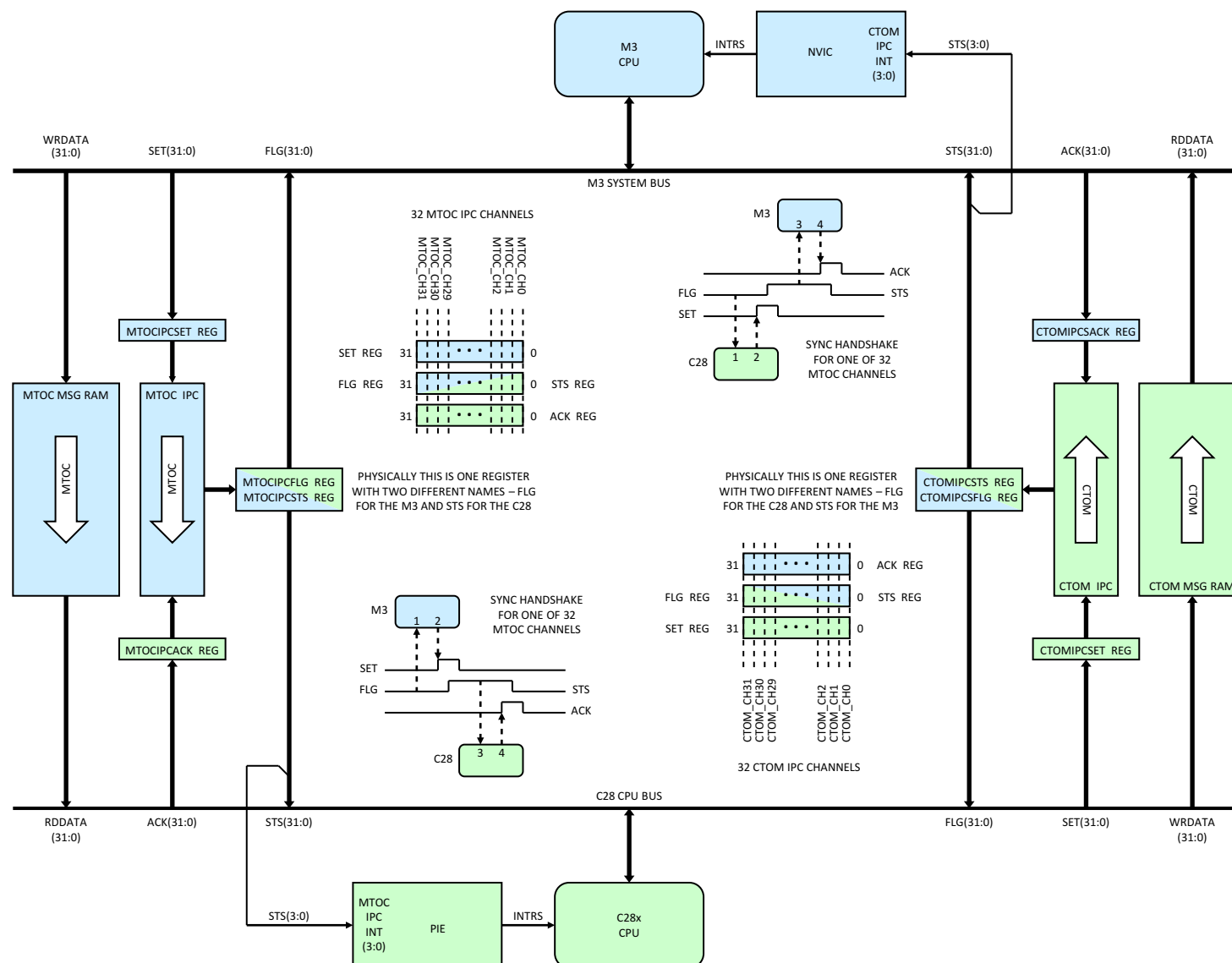
Figure 5-16. IPC
