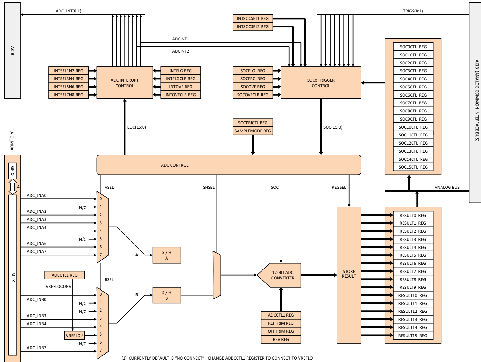
Figure 5-11. ADC
