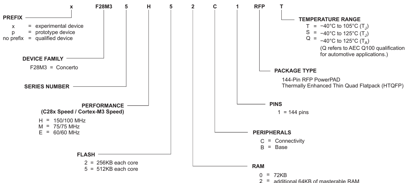
Figure 8-1. Device Nomenclature
