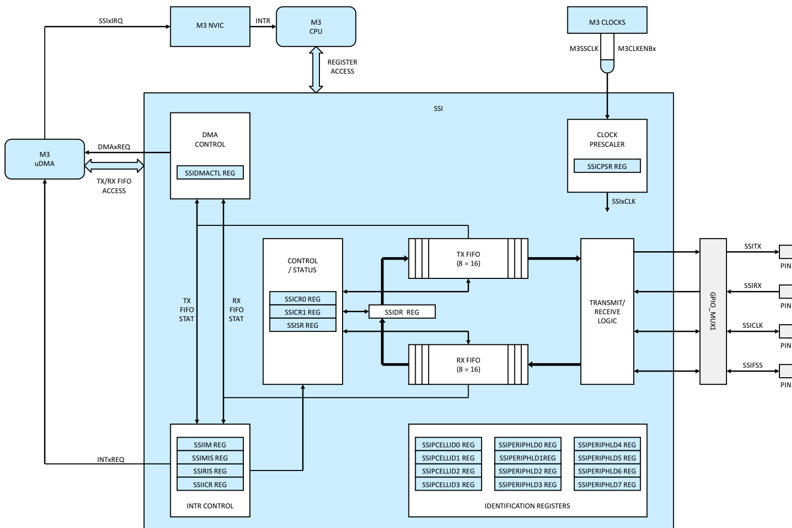
Figure 5-31. SSI
