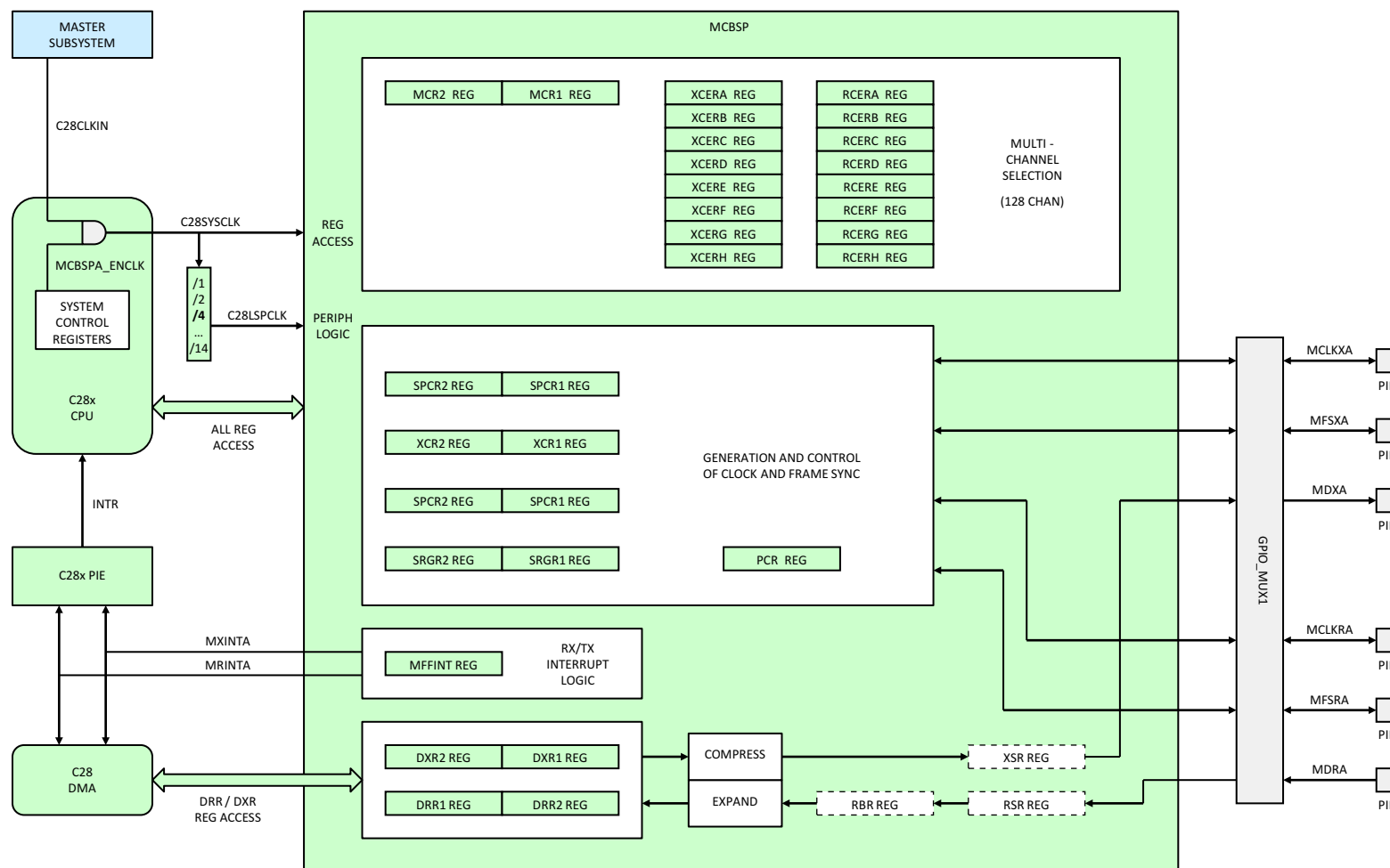
Figure 5-56. McBSP (C28x)
