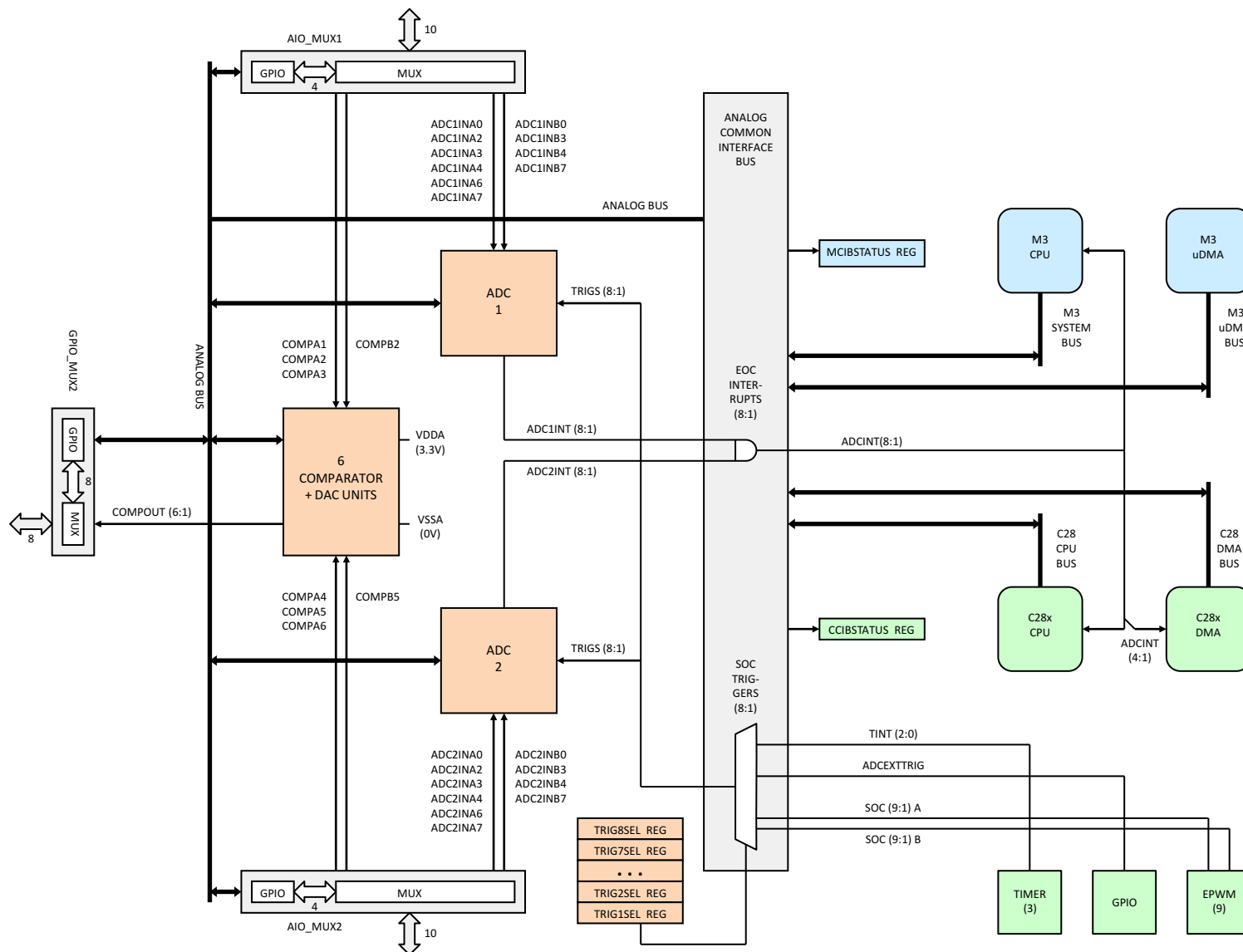
Figure 6-3. Analog Subsystem
