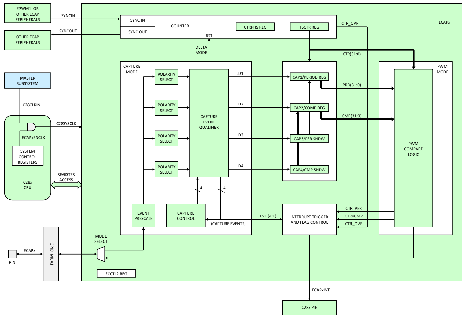
Figure 5-47. eCAP
