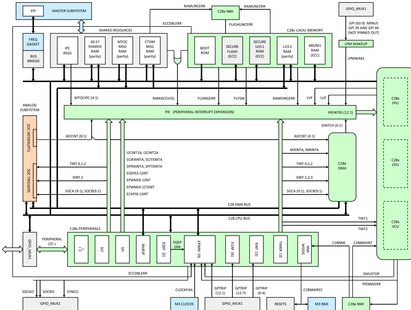
Figure 6-2. Control Subsystem
