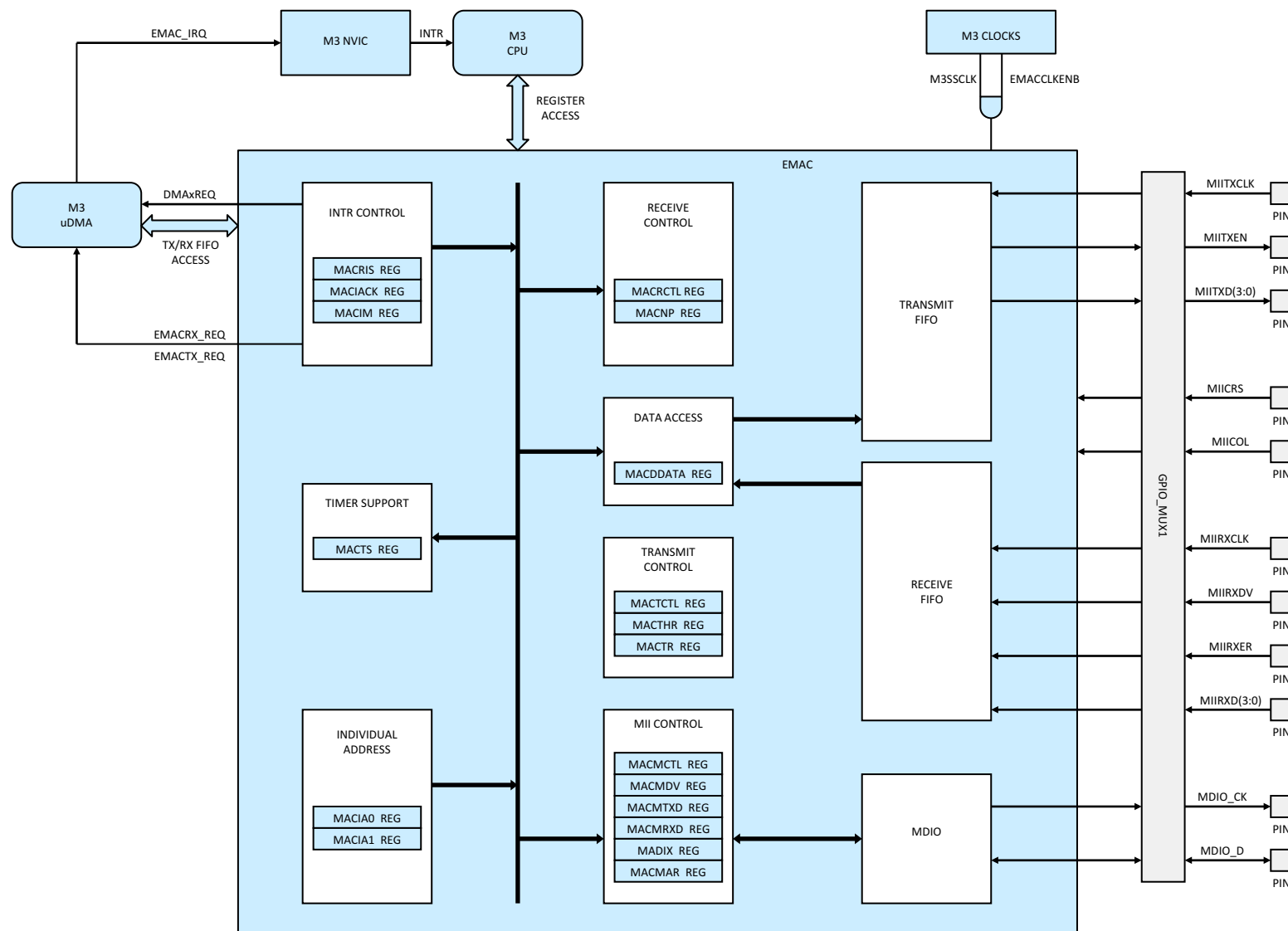
Figure 5-36. EMAC
