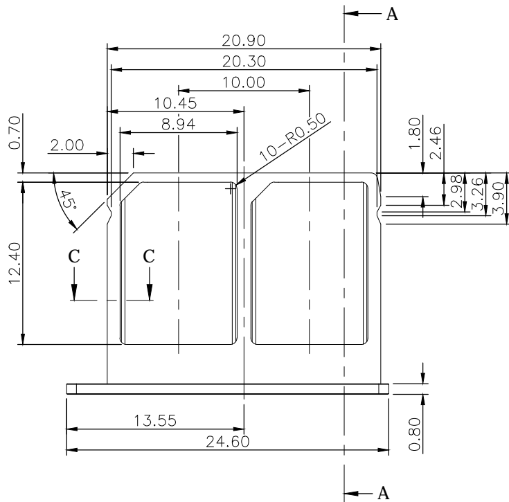
DETAIL D Scale 10/1
