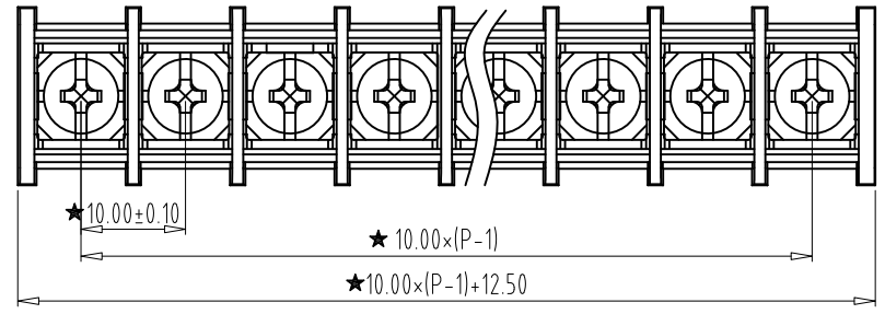
PCB LAYOUT
