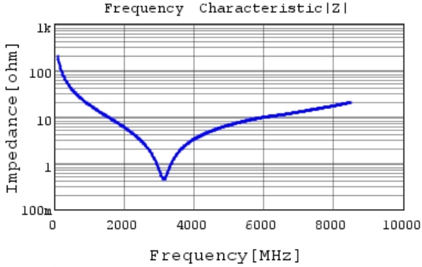
GRM1555C1H8R0BA01 |Z| DCOV, 25degC
