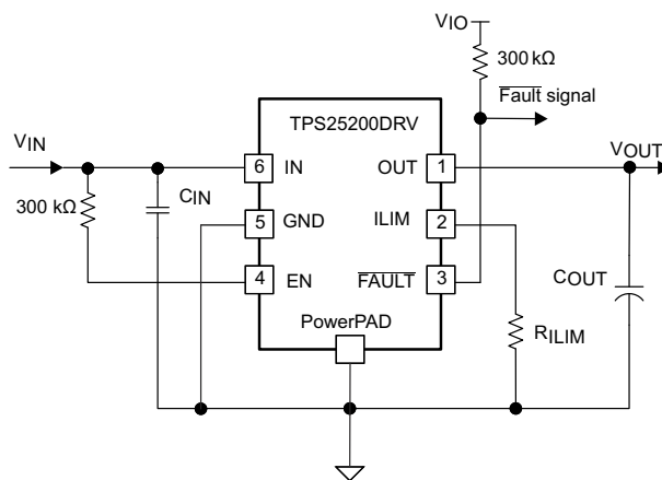
Simplified Schematic
