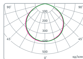
NHB-P5-100-5K-120D-LED
