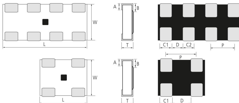
(2) Inverted Type Array
