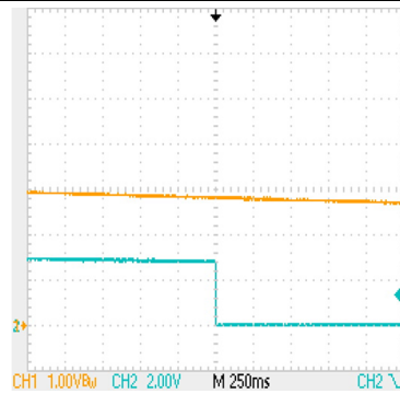
Orange Line (Channel 1) = Power Down Ramp on BAT Pin Turquoise Line (Channel 2) = DOUT Date Drive Output DOUT goes from high to low when UVP threshold = UVP set Threshold + set delay time
