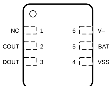
DSE Package 6-PIN WSON Top View
