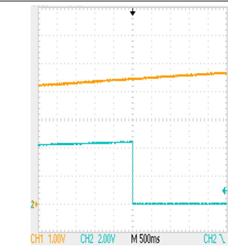
Orange Line (Channel 1) = Power Up Ramp on BAT Pin Turquoise Line (Channel 2) = COUT Gate Drive Output COUT goes from high to low when OVP threshold = OVP set Threshold + set delay time
