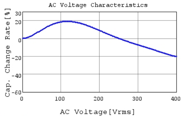
RDER73A104K5E1H03A C-AC Voltage capchange, I
