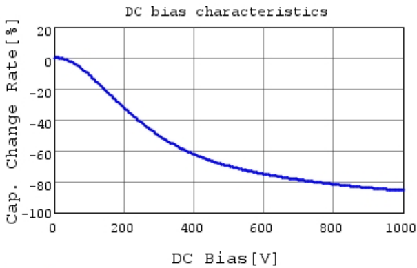
RDER73A104K5E1H03A C-DC bias capchange, 25.0
