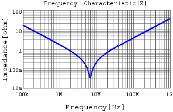
RDER73A104K5E1H03A |Z| DCOV, 25degC
