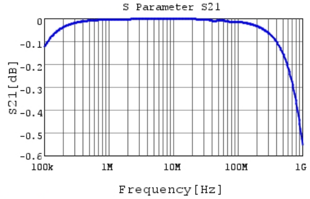
RDER73A104K5E1H03A S21 DCOV, 25degC
