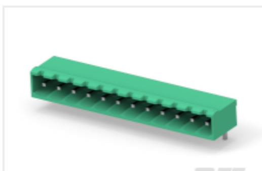
TE Part #1-2350513-2 12POS TB HDR 90 DEG, PITCH 5.0 & TL 4.5mm
