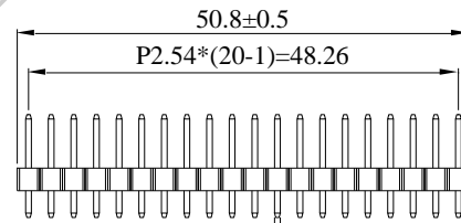
Pin Detail SCALE 1/1
