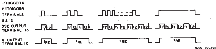
Fig. 34—Retrigger-mode waveforms.
