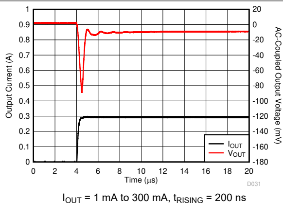
Figure 6-53. Load Transient
