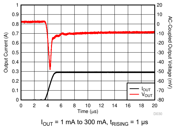
Figure 6-51. Load Transient
