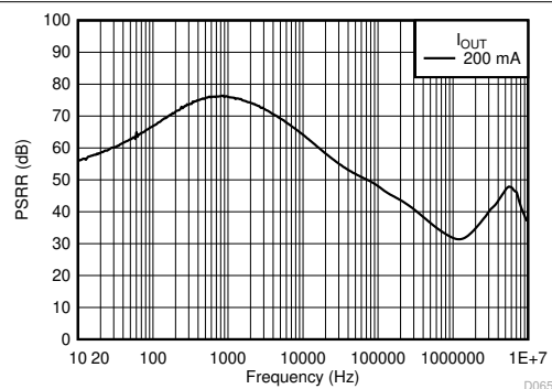
Figure 8-6. PSRR
