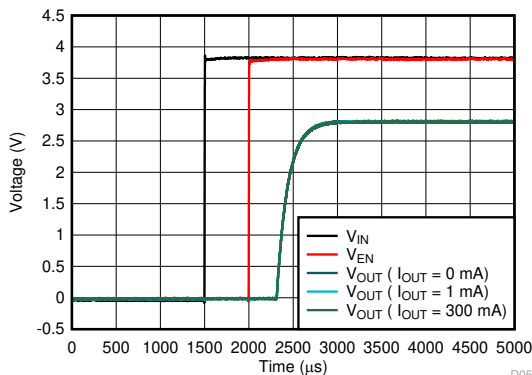
Figure 6-75. Start-Up
