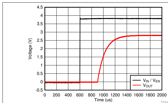
Figure 8-5. Start-Up
