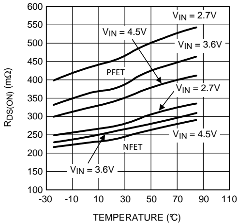
Figure 7. R_{DS(on)} vs Temperature
