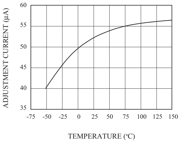
Fig3. Adjustment Current
