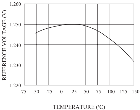
Fig5. Temperature Stability
